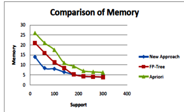
Figure 3.2: The memory usage at various support levels on dataset
