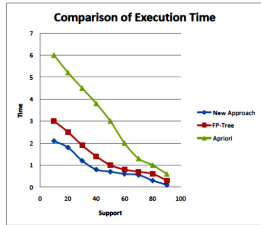
Figure 3.1: Execution Time for Artificial dataset
