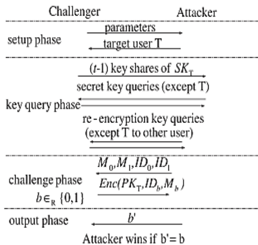
Figure 2. The security game for the chosen plaintext attack.
