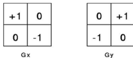
Figure 2. Robert Cross kernel
