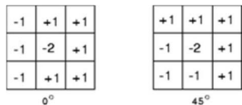
Figure 3. Prewitt Mask
