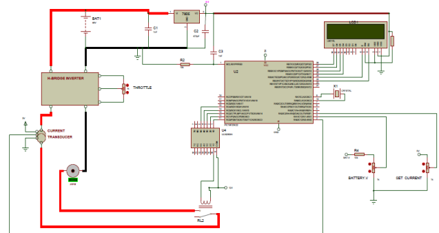
Figure 3. Circuit Diagram
