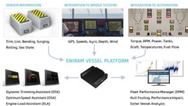
Figure 2. Ship Automation System Data Collection for Analysis.
