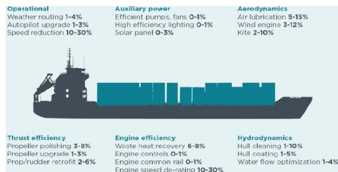
Figure 1. Potential Fuel use and CO2 reduction from various energy Efficiency Approaches for Ship - International Council on clean transport July 2013.
