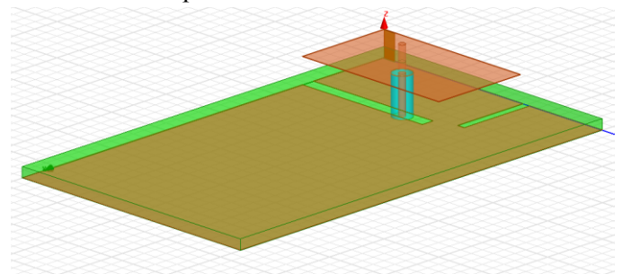
Figure 1. 3D view of proposed antenna.
