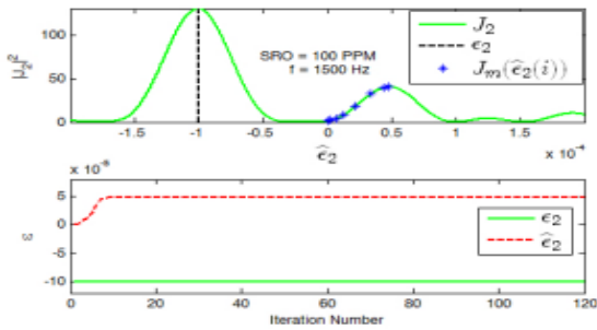
Fig. 3. Gradient Ascent trapped in a local maximum due to poorly chosen initial conditions. Noticed that the slant of the cost work is getting moderate once a low recurrence band is considered, which additionally hampers the estimation execution. The above perceptions direct that a legitimate recurrence choice philosophy is required with a specific end goal to effectively gauge the SROs utilizing the proposed iterative technique. Be that as it may, such a procedure is past the extent of the present commitment and will be a subject for a future report.
