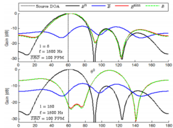
Fig. 1. Empirical vs. analytical beampatterns of SDBF
