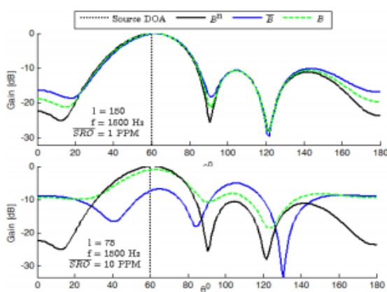
Fig. 2: SDBF beam patterns for various SROs
