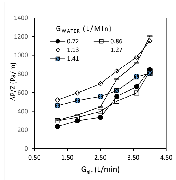
Figure 3 –Pressure drop variation with the air flow
