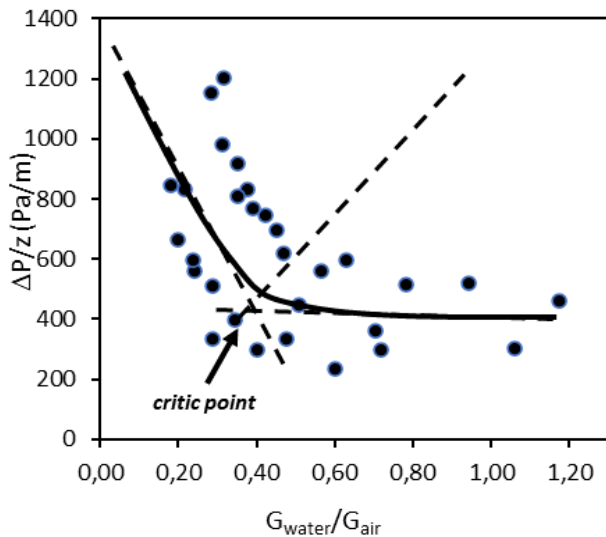
Figure 6 - Pressure drop variation against G_{\text{water}}/G_{\text{air}} and the critic point.
