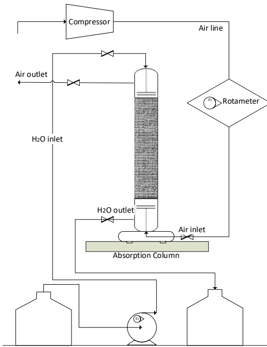
Figure 1 - The experimental installation
