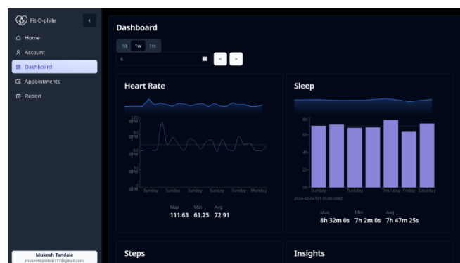
Fig 4: Dashboard
