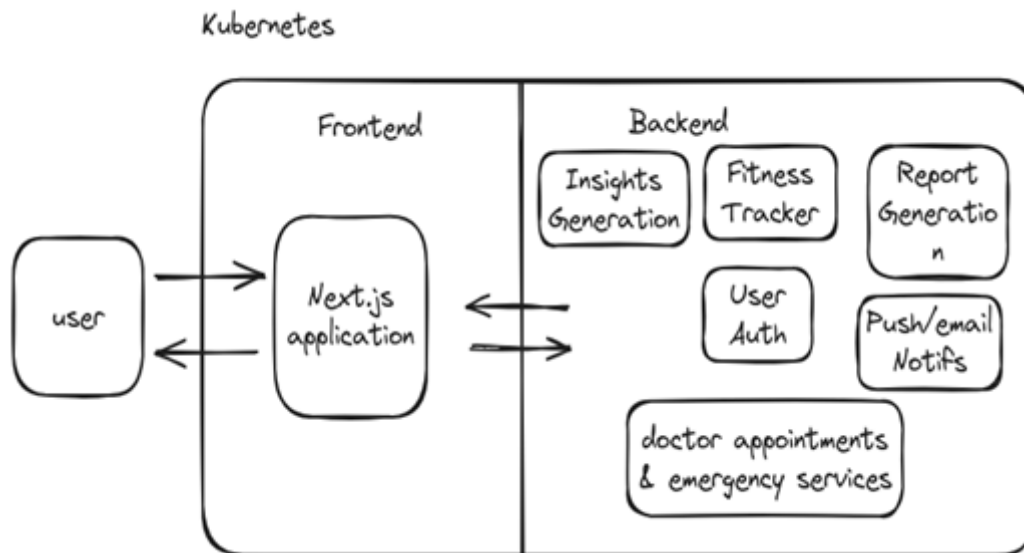
Fig 1: Architecture diagram
