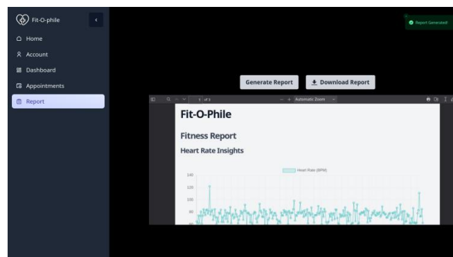
Fig 5: Report Page
