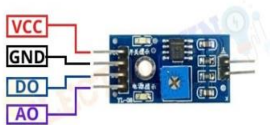
Figure 6: Moisture Sensor
