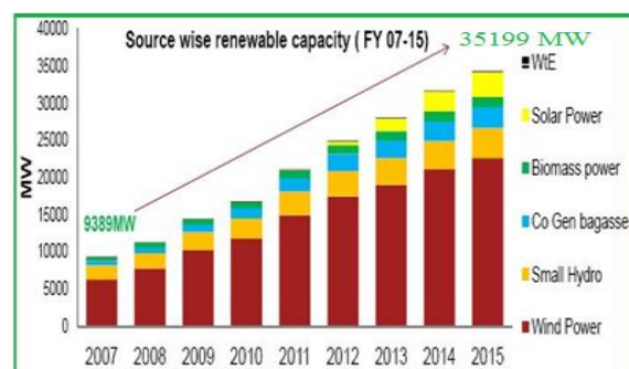
Figure5. The source wise Renewable Energy status
