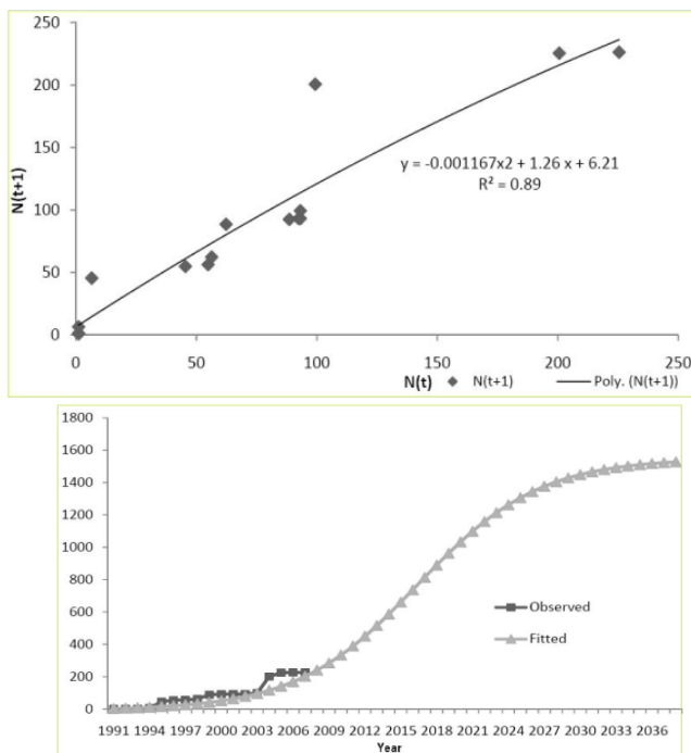
Figure 11. Cumulative wind power installations (MW) (Best Fit for p=0.001 , q=0.196 , m=1550 )
