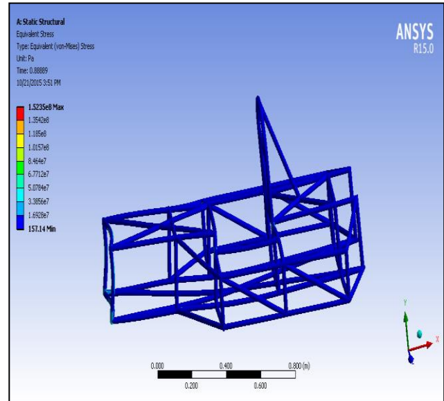
Figure 5. Equivalent Stress
