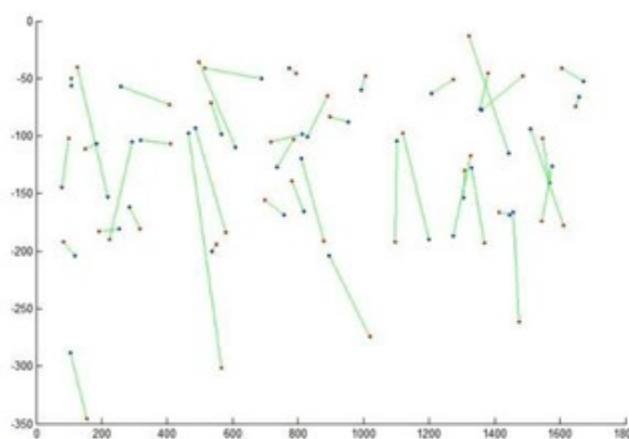
Figure 8 : Red indicates true click position, and blue indicates the system's predicted eye gaze location at the time of that click. The prediction is made by transforming pupil offset with the H matrix discussed previously
