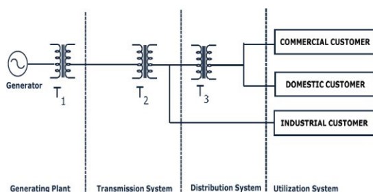
Figure 1. Typical Power System
