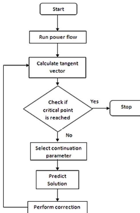
Figure 2 : Flow Chart for Continuation Power Flow [20]
