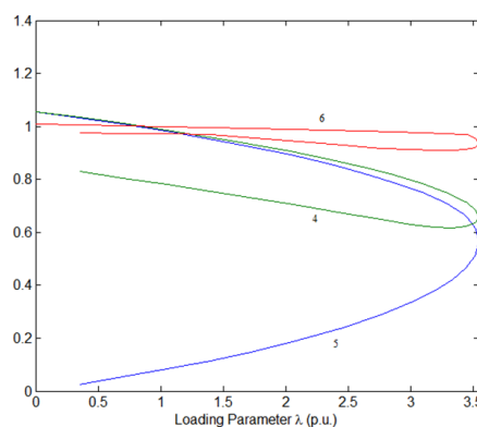
Figure 4. P-V Curves with STATCOM at Bus 6 Maximum Loading Value after CPF with STATCOM at Bus 6 \lambda = 3.5429
