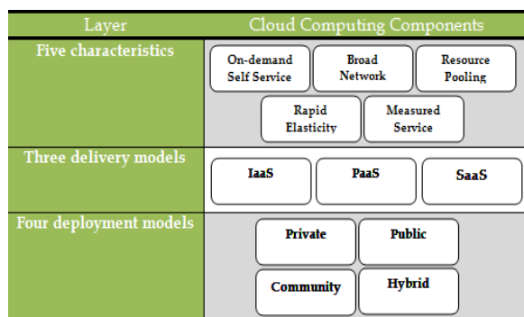
Figure 1: Cloud Computing
