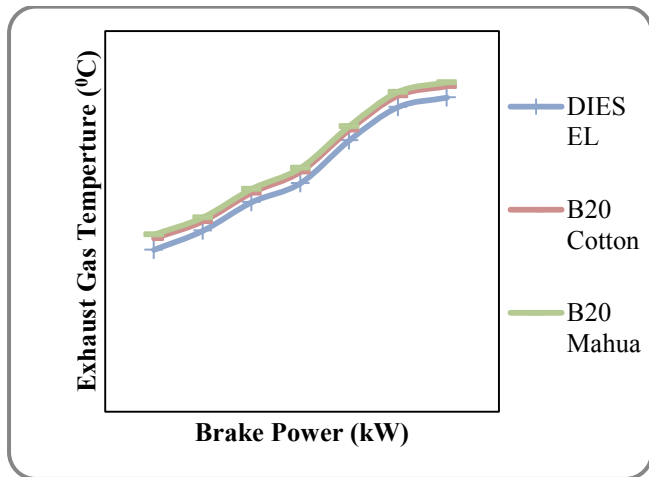
Figure 3. The variation of EGT with brake power
