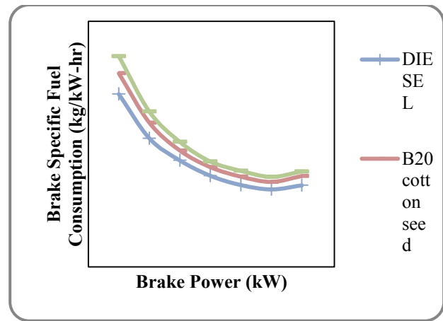
Figure 2. The variation of BSFC with brake power
