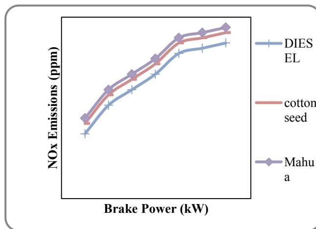
Figure 7. The variation of Nitrogen oxide emissions
