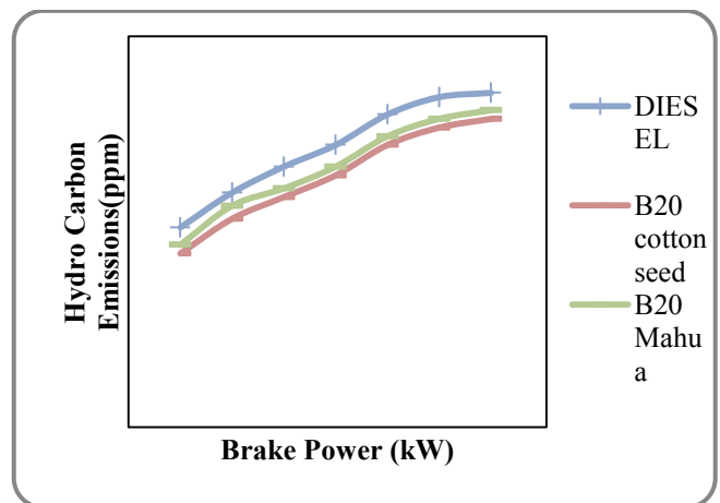
Figure 5. The variation of HC emissions with brake power
