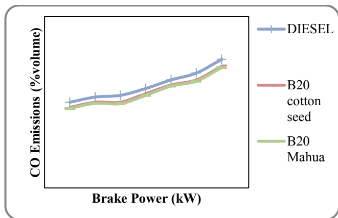
Figure 6. The variation of CO emissions with brake power
