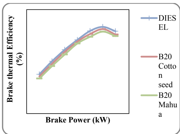
Figure 1. The variation of Brake thermal efficiency
