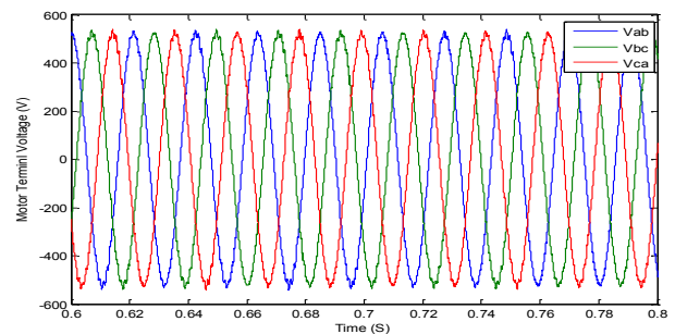
Figure 8(a). Output voltage waveform
