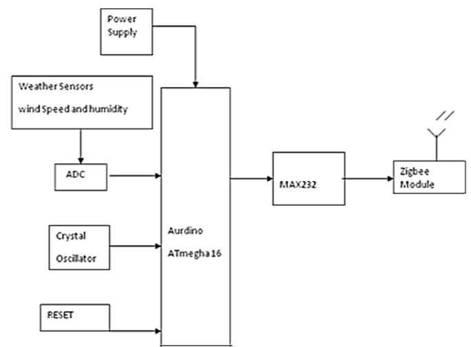
Fig1. Transmitter Circuit.
