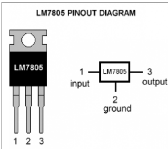
Fig.4 voltage regulator
