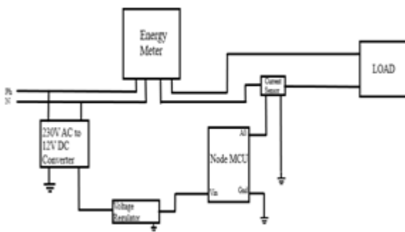
Fig.5 Block Diagram of IOT Based Smart Energy Meter
