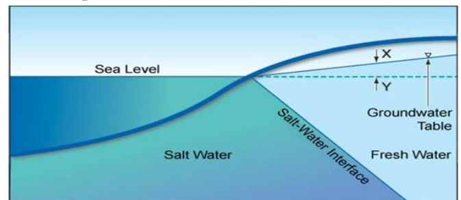
Figure 1: Salt-water interface in an unconfined coastal aquifer according to the Ghyben-Herzberg relation. (X Groundwater Level, Y Sea water Level) (Courtesy: www.solinst.com )
