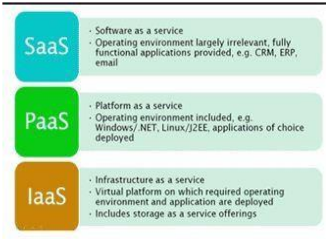
Figure 2 : Basic Cloud Service models
