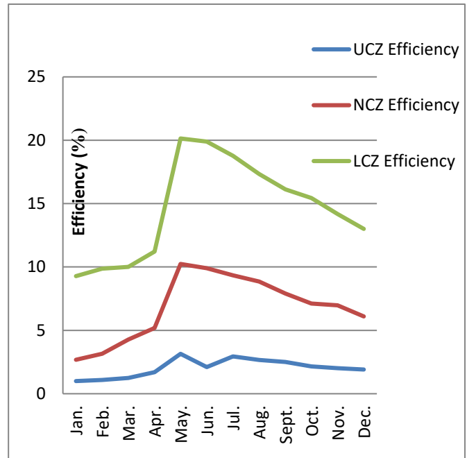
Figure 2: Variations of exergy efficiencies of the solar pond in a year
