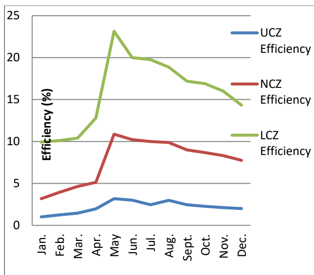
Figure 1: Variations of energy efficiencies of the solar pond in a year
