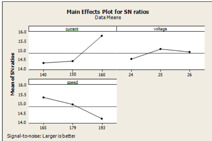
Fig 1 : Main Effect plot for S/N Ratio
