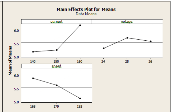
Fig 2 : Main Effect plot for Mean
