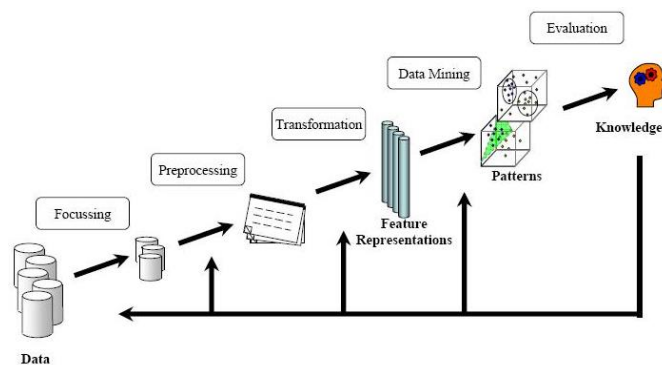
Figure 1 : KDD Process
