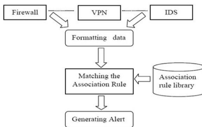
Fig. 3. Framework of the association analysis
