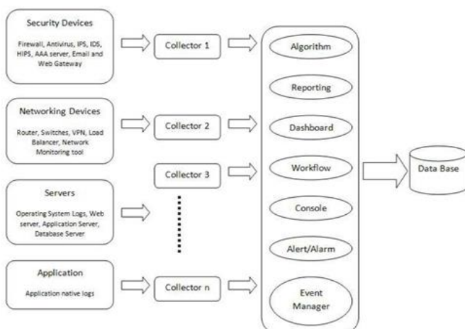
Fig. 2. SIEM architecture
