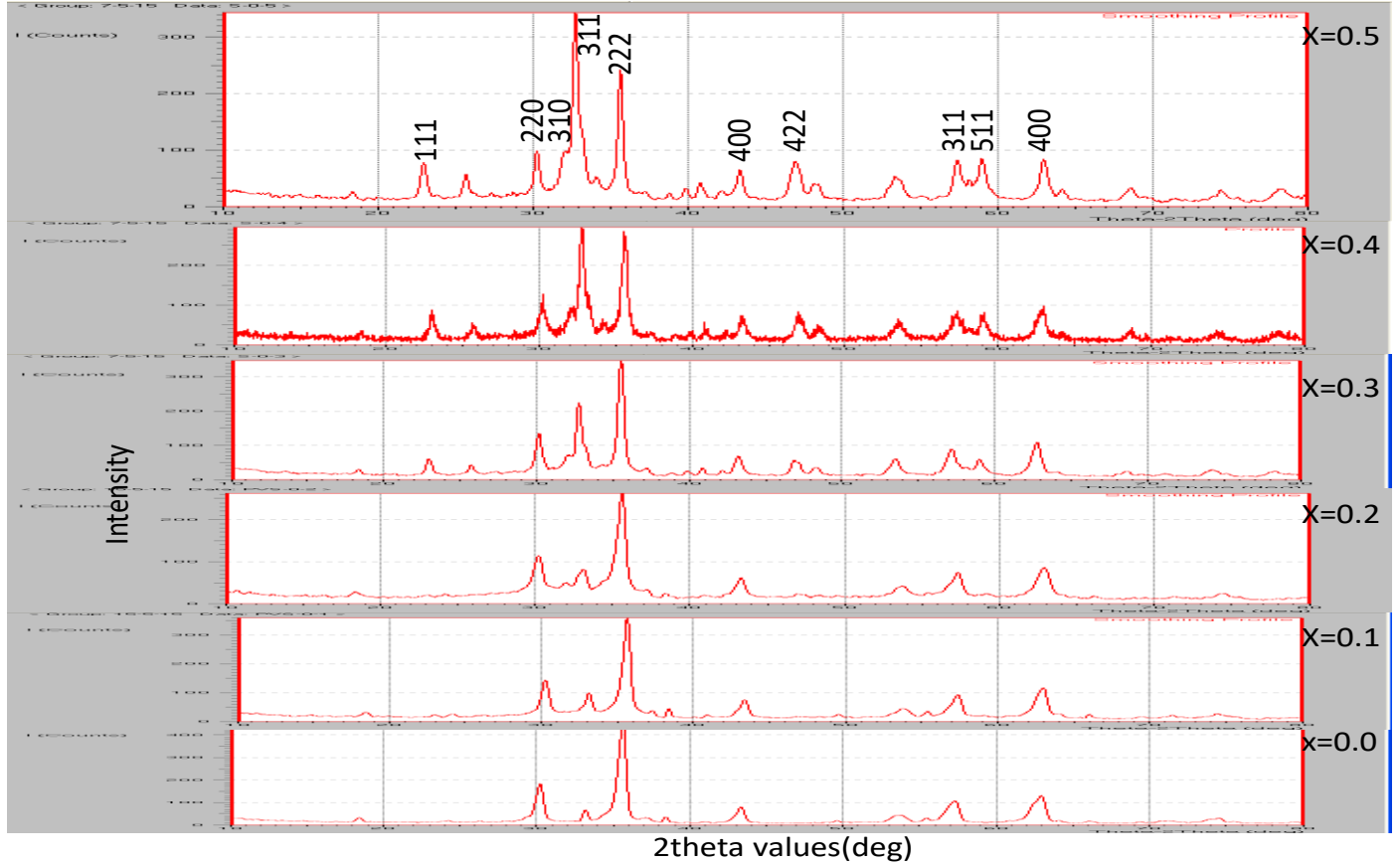
Fig (1). XRD Pattern of Sm substituted Ni Cd nano Ferrite
