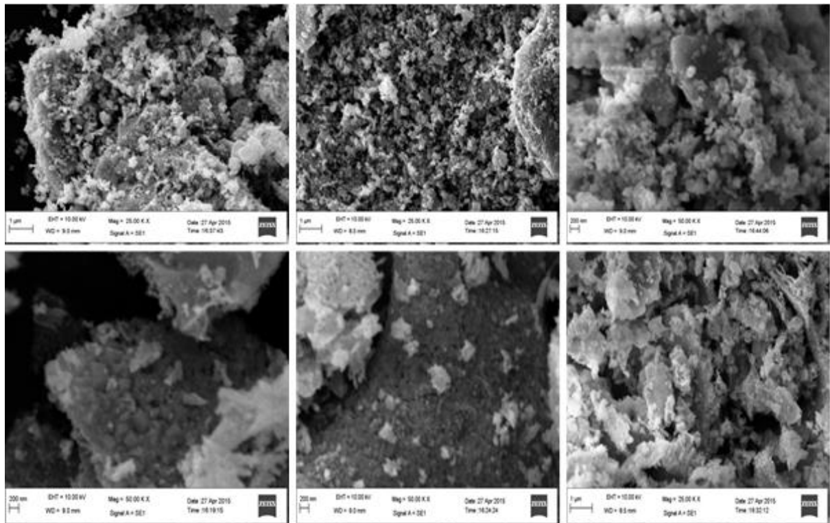
Fig (2). SEM Micro graphs of Ni Cd Sm nano ferrites
