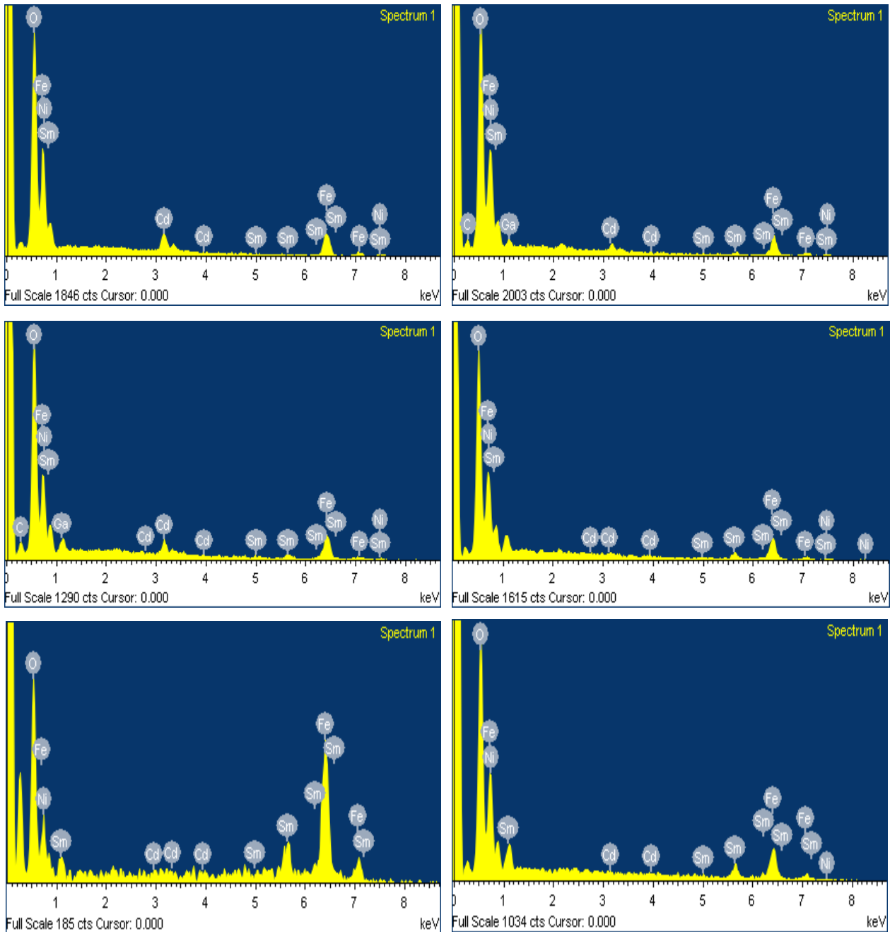
Fig (3). EDS Patron of Ni Cd Sm x Fe 2-x O 4 with x = 0.0, 0.1, 0.2, 0.3, 0.4, 0.5.
