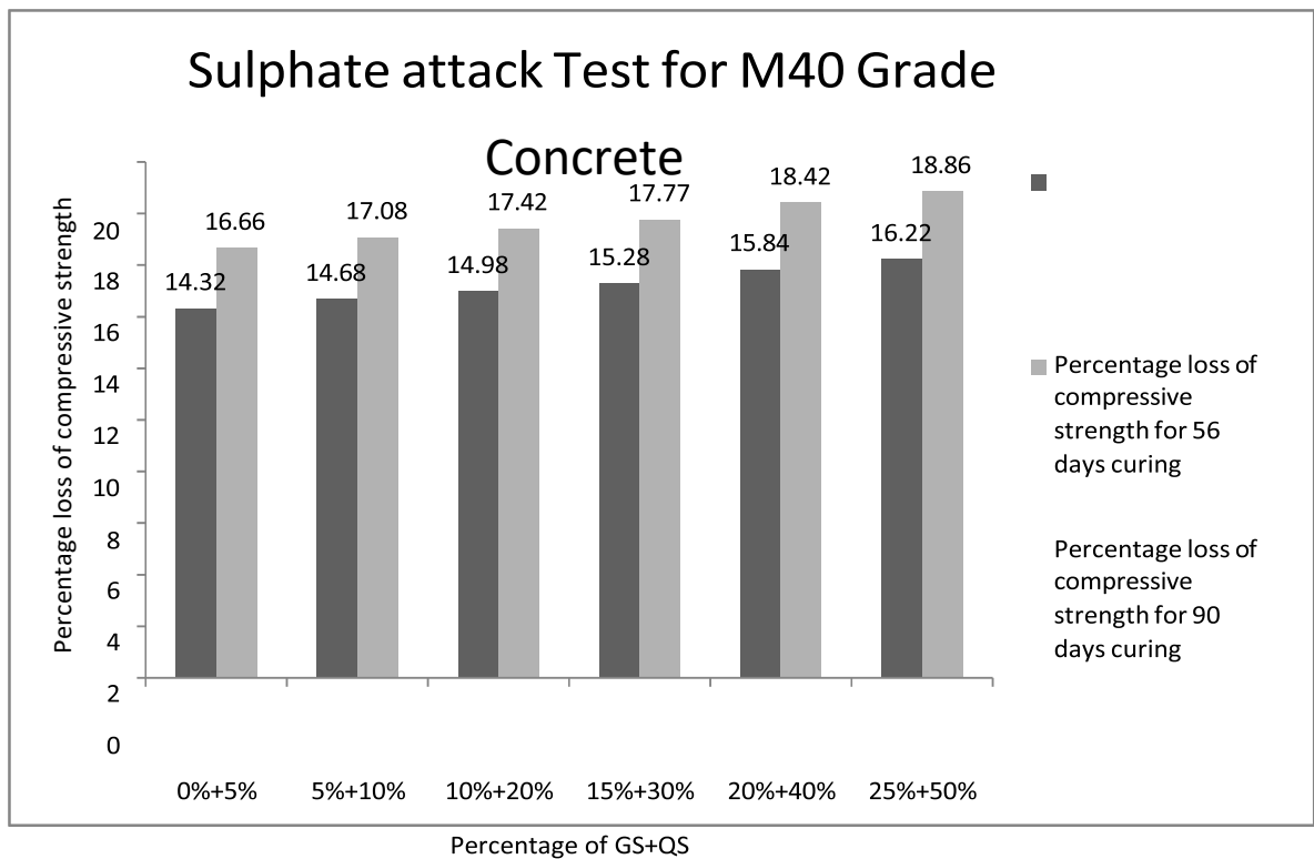
Fig Sulphate attack for M40 Grade Concrete
