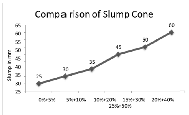
Fig Slump Cone Test for M40 Grade concrete
