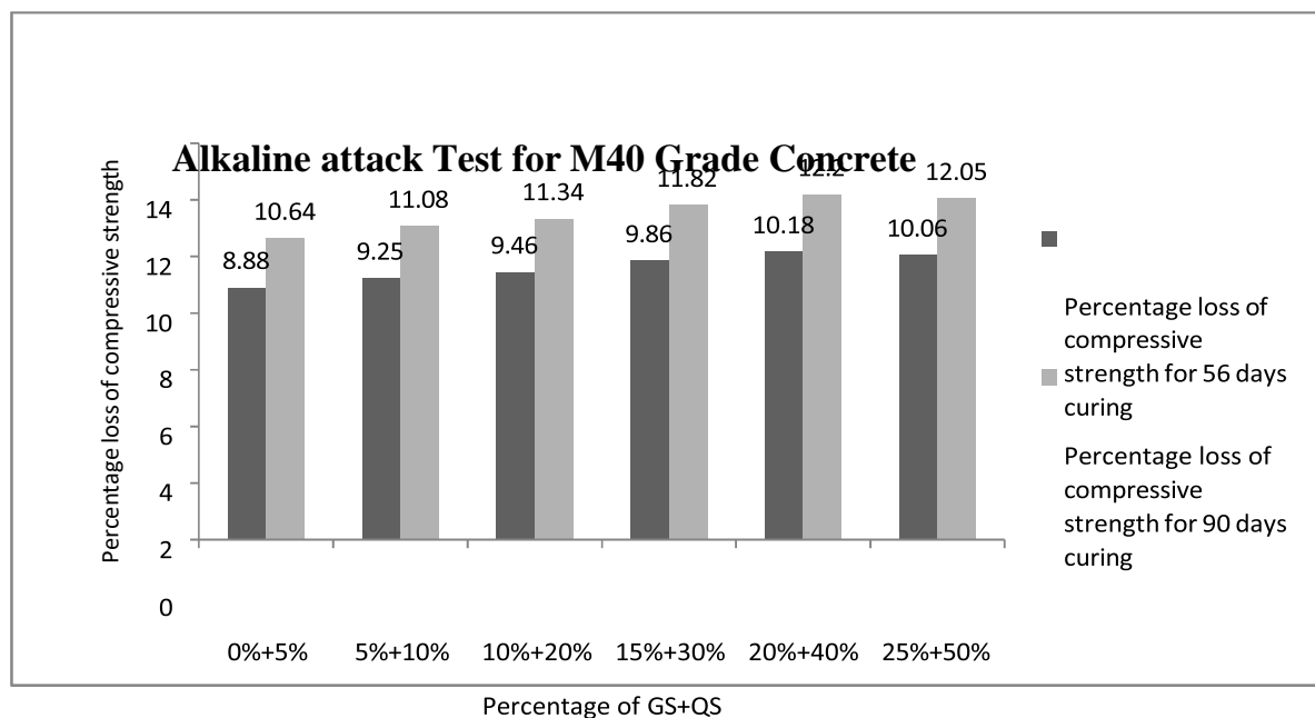
Fig Alkaline attack for M40 Grade Concrete
